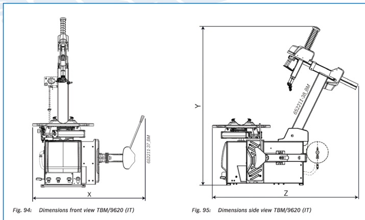
Image shows tyre changer with optional Technoroller
